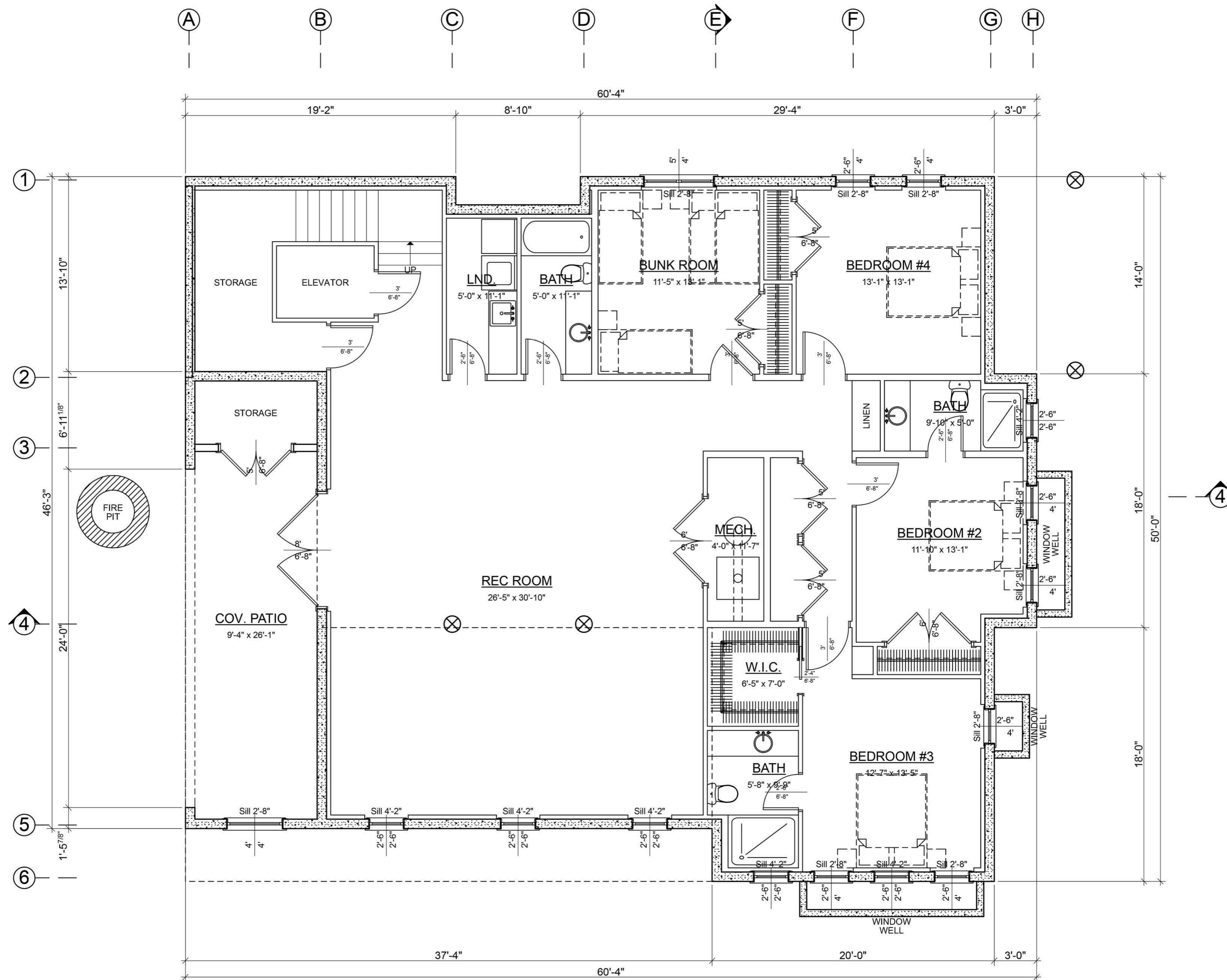
Sierra Blanca: BASEMENT FLOOR PLAN SCALE: 1/4" = 1'-0" AREA: 2467 sq ft
